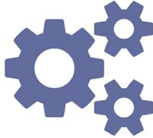
Business Rules
